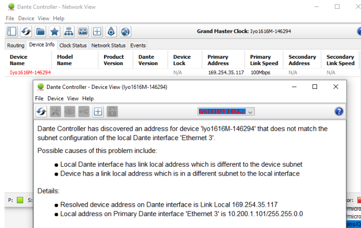
Figure 2 Dante Controller Iyo subnet mismatch
