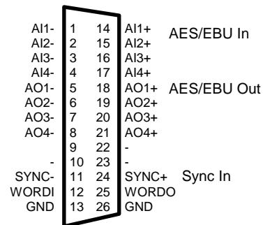
High Density 26pin
