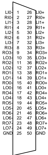
Centronics 50pin
