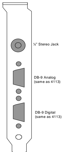
ASI5111 Connectors
